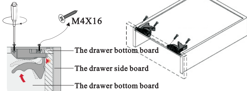
Drawer handle installation
